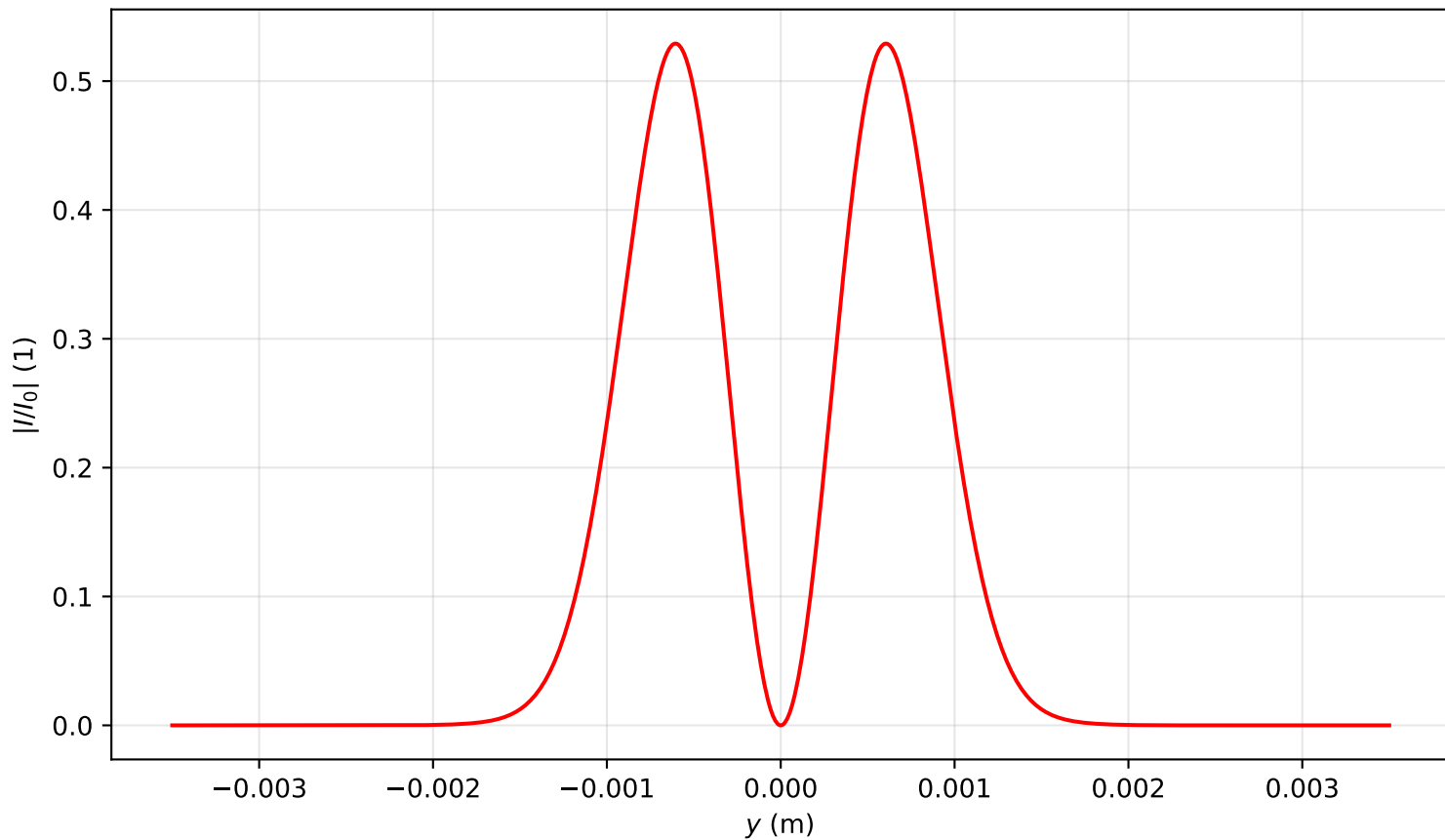
Intensity profile I(x=0, y, z=1.353)/I_0 , P_{in}=0.5P_{cr} , artificial time
